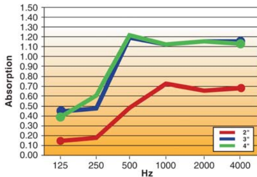
FOAM S.T.O.P. Pyramid – Sound Absorption/Noise Reduction
