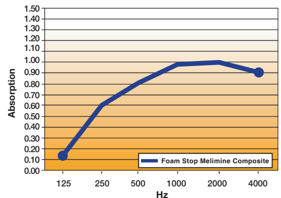
Sound Absorption Coefficients - Type B Mtg. - ASTM C423-90A
